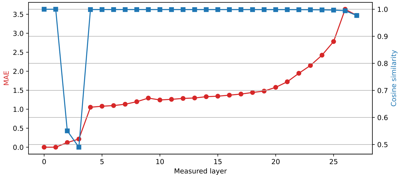
Qwen2.5-7B-Instruct | Quantized layer 1 | float64 → int2
