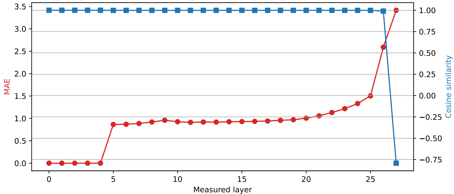
Qwen2.5-7B-Instruct | Quantized layer 4 | float64 → int2
