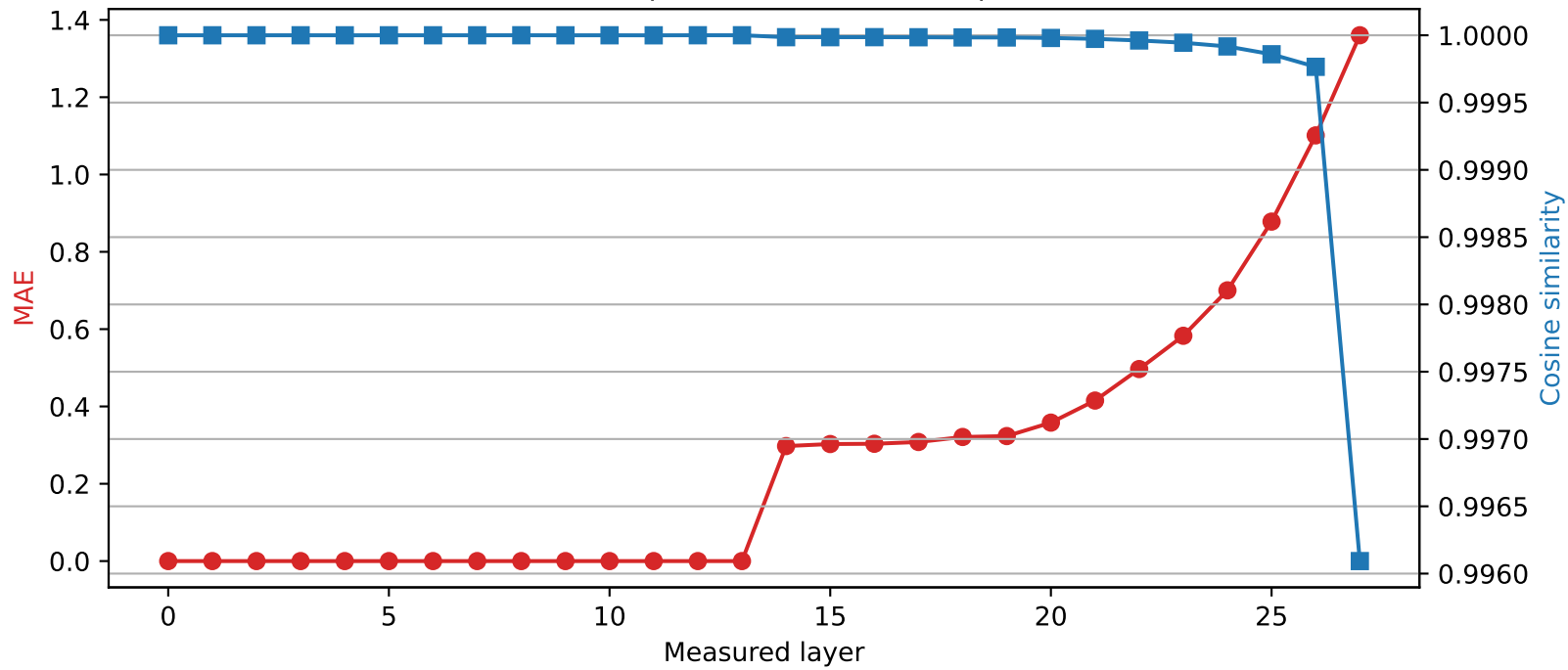
Qwen2.5-7B-Instruct | Quantized layer 13 | float64 \rightarrow int2
