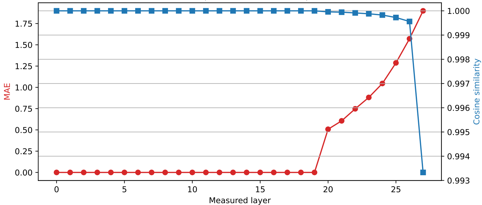
Qwen2.5-7B-Instruct | Quantized layer 19 | float64 \rightarrow int2
