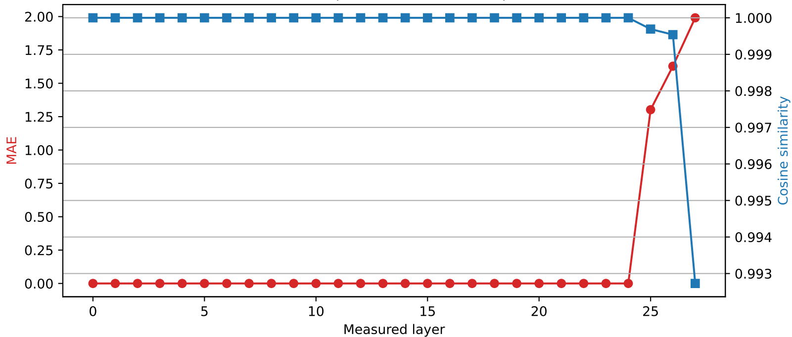
Qwen2.5-7B-Instruct | Quantized layer 24 | float64 \rightarrow int2
