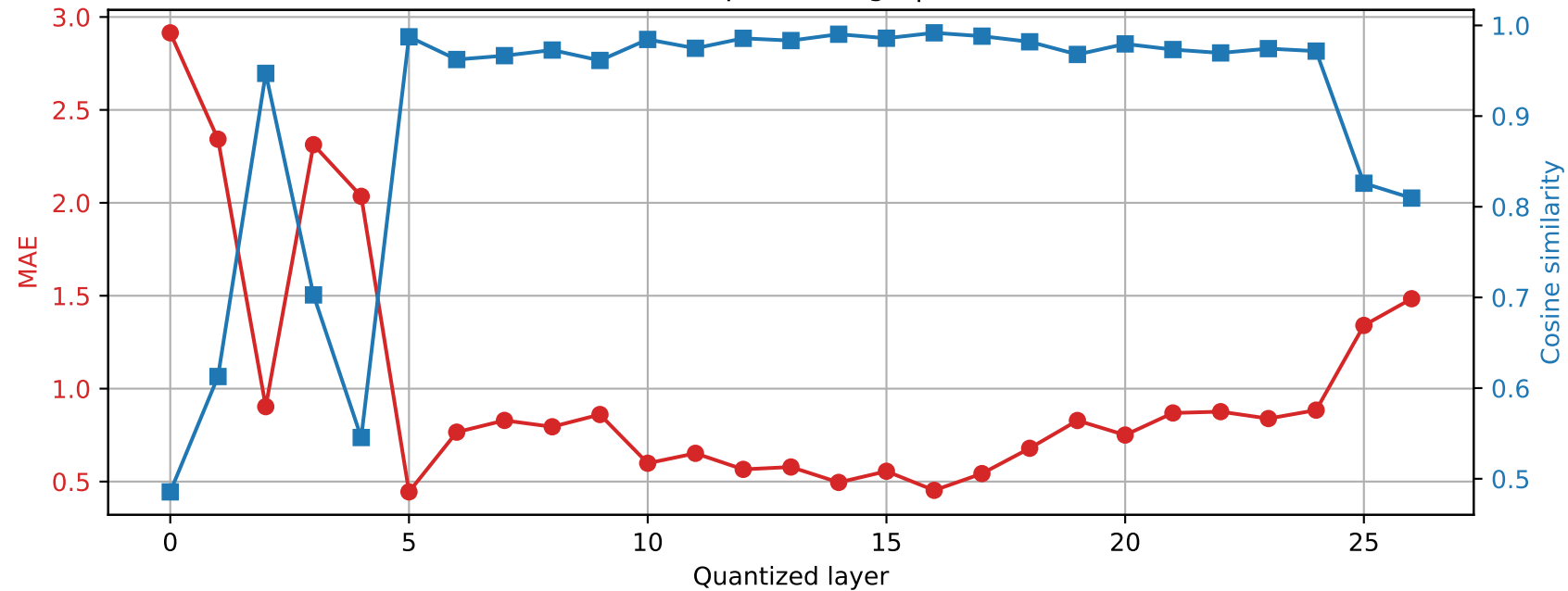
Qwen2.5-7B-Instruct | Prompt 2 Final RMSNorm output damage | float64 \rightarrow int2
