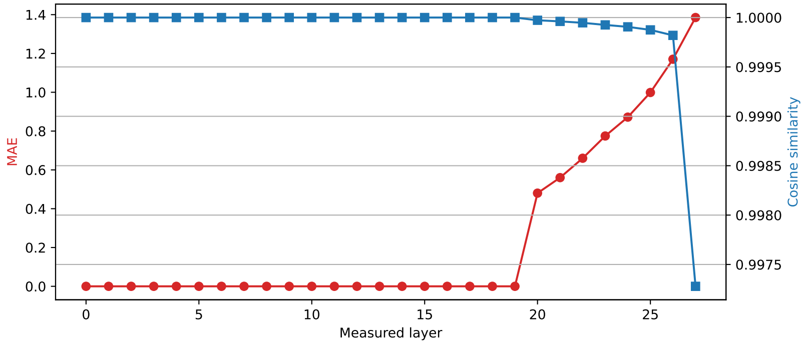
Qwen2.5-7B-Instruct | Quantized layer 19 | float64 → int2
