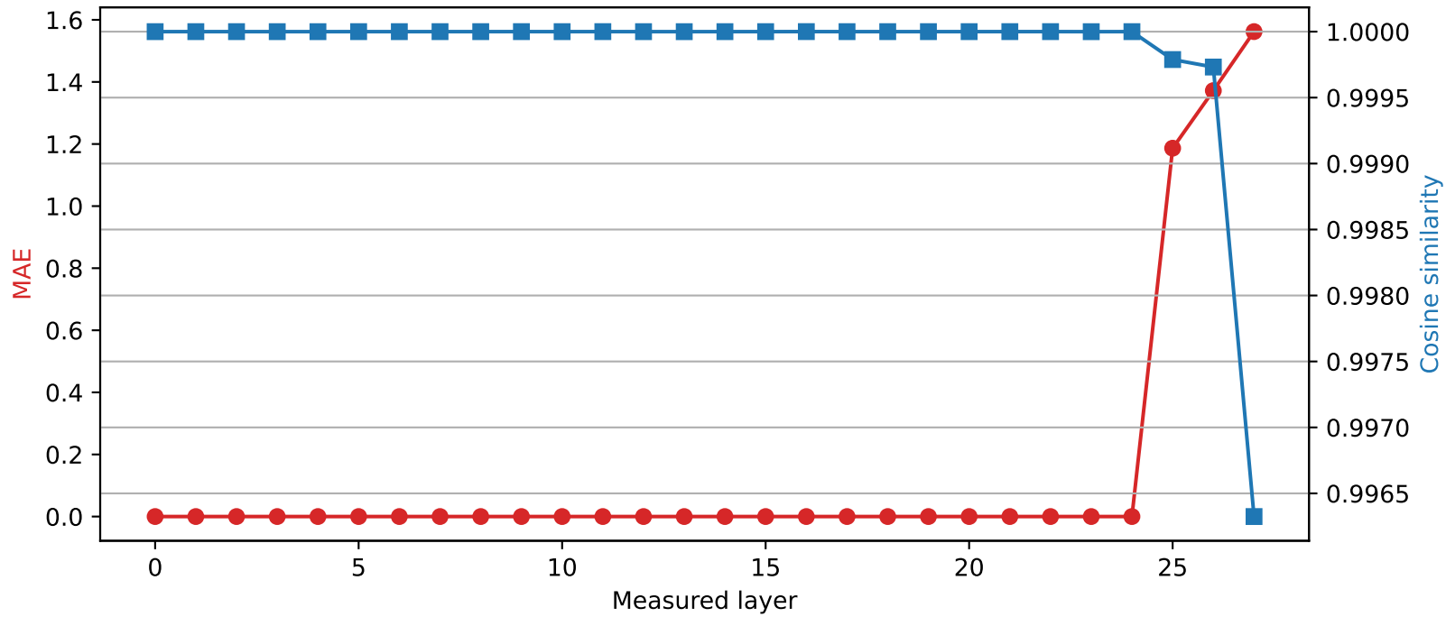
Qwen2.5-7B-Instruct | Quantized layer 24 | float64 → int2
