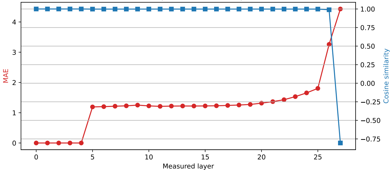
Qwen2.5-7B-Instruct | Quantized layer 4 | float64 \rightarrow int2
