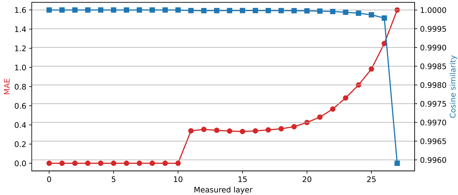
Qwen2.5-7B-Instruct | Quantized layer 10 | float64 → int2
