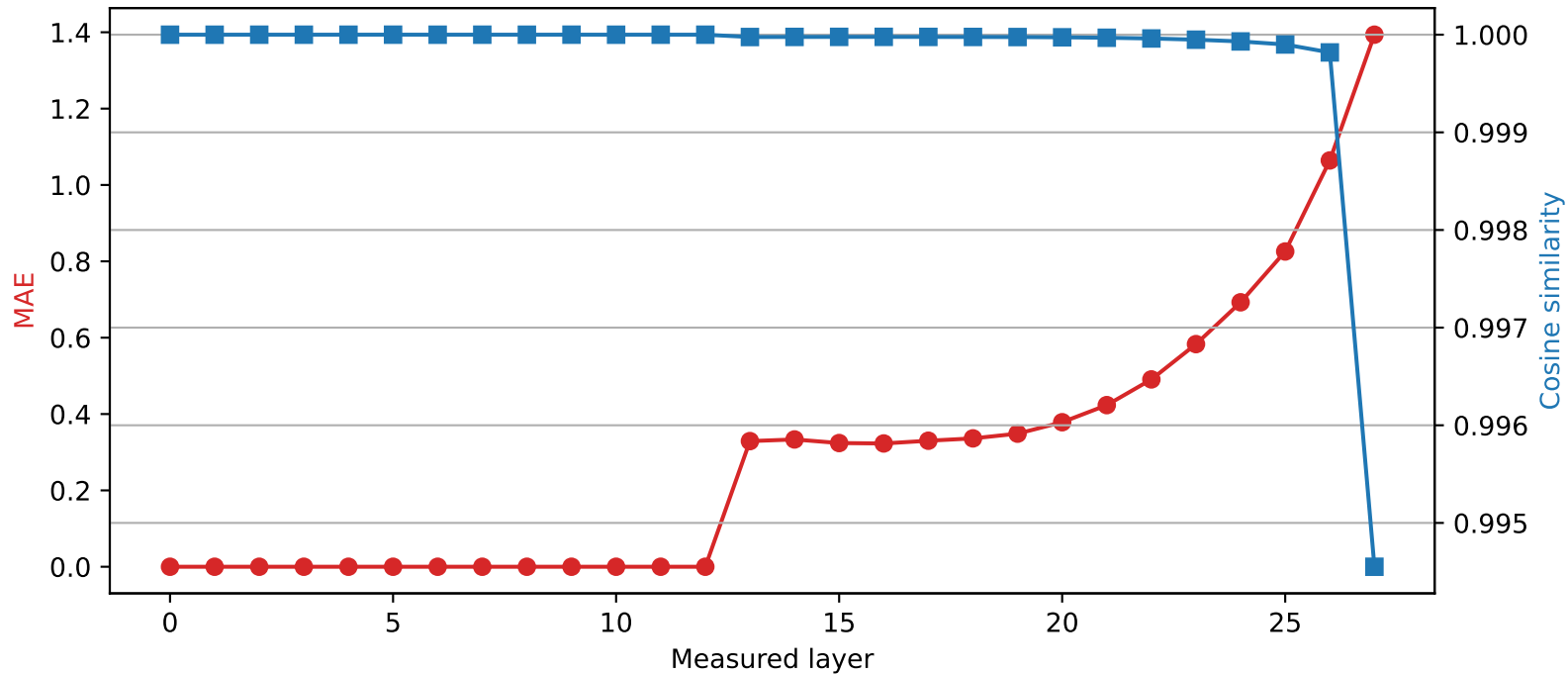
Qwen2.5-7B-Instruct | Quantized layer 12 | float64 \rightarrow int2
