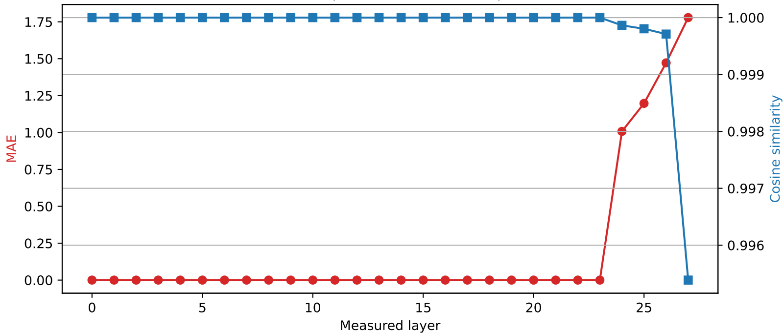
Qwen2.5-7B-Instruct | Quantized layer 23 | float64 → int2
