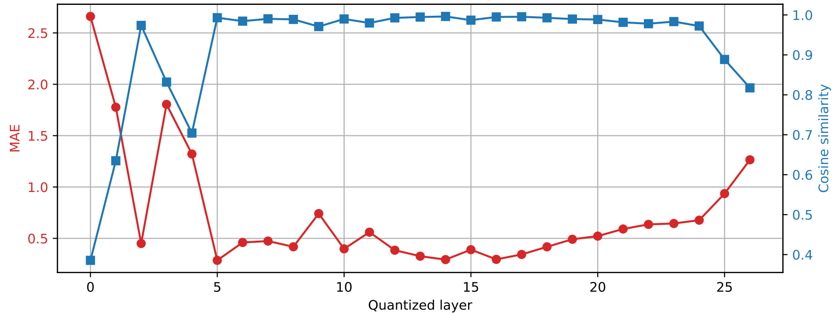
Qwen2.5-7B-Instruct | Prompt 4 Final RMSNorm output damage | float64 \rightarrow int2
