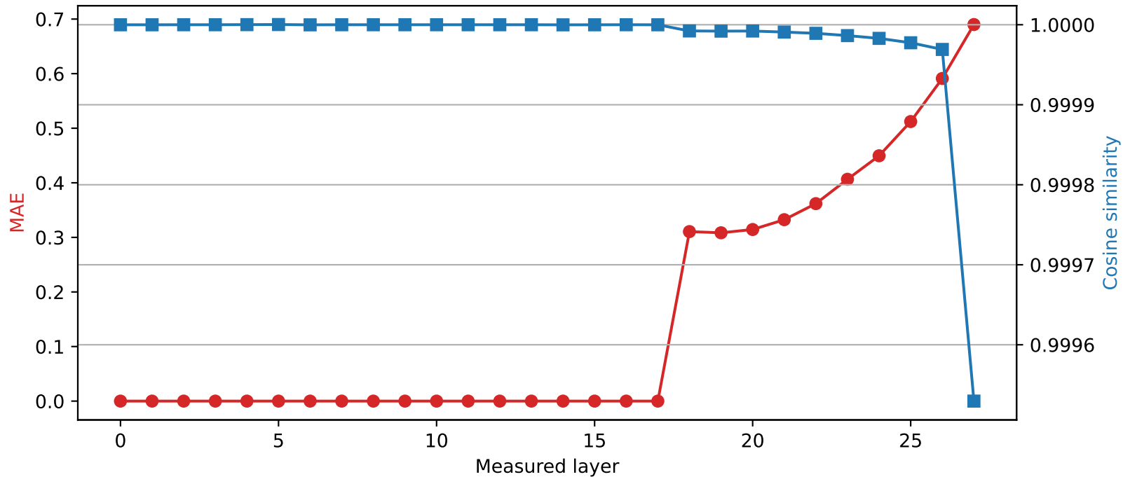
Qwen2.5-7B-Instruct | Quantized layer 17 | float64 → int2
