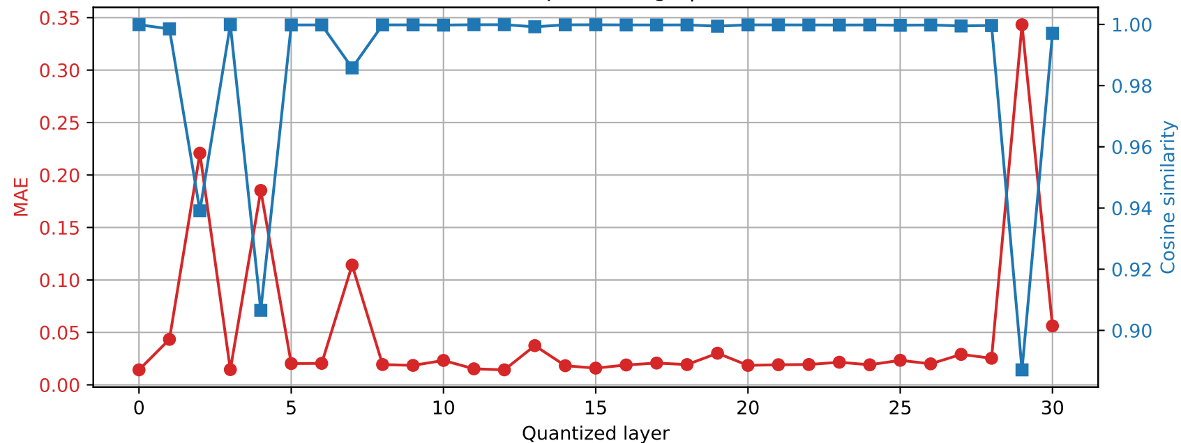
Phi-3-mini-4k-instruct | Prompt 0 Final RMSNorm output damage | float16 \rightarrow int8
