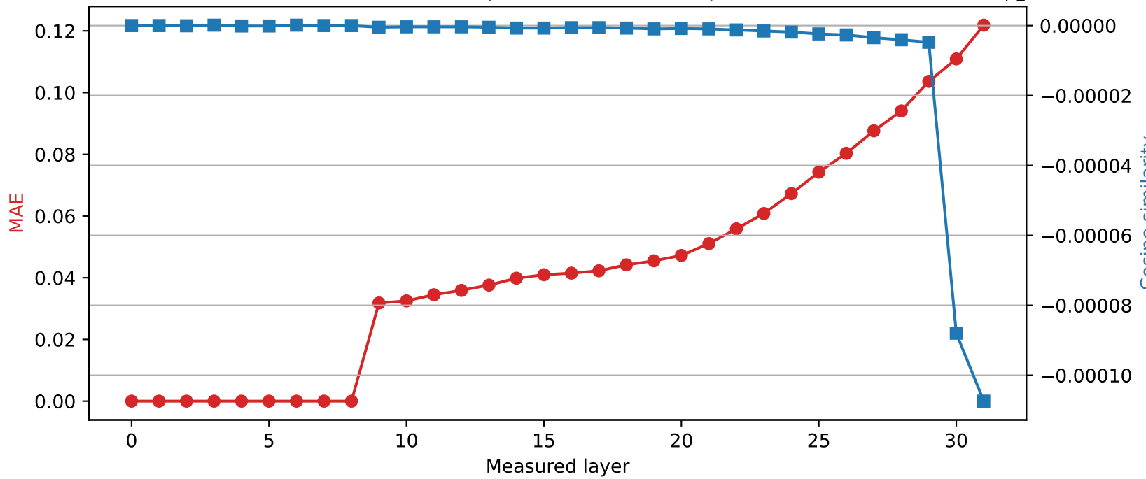
Phi-3-mini-4k-instruct | Quantized layer 8 | float16 \rightarrow int8
