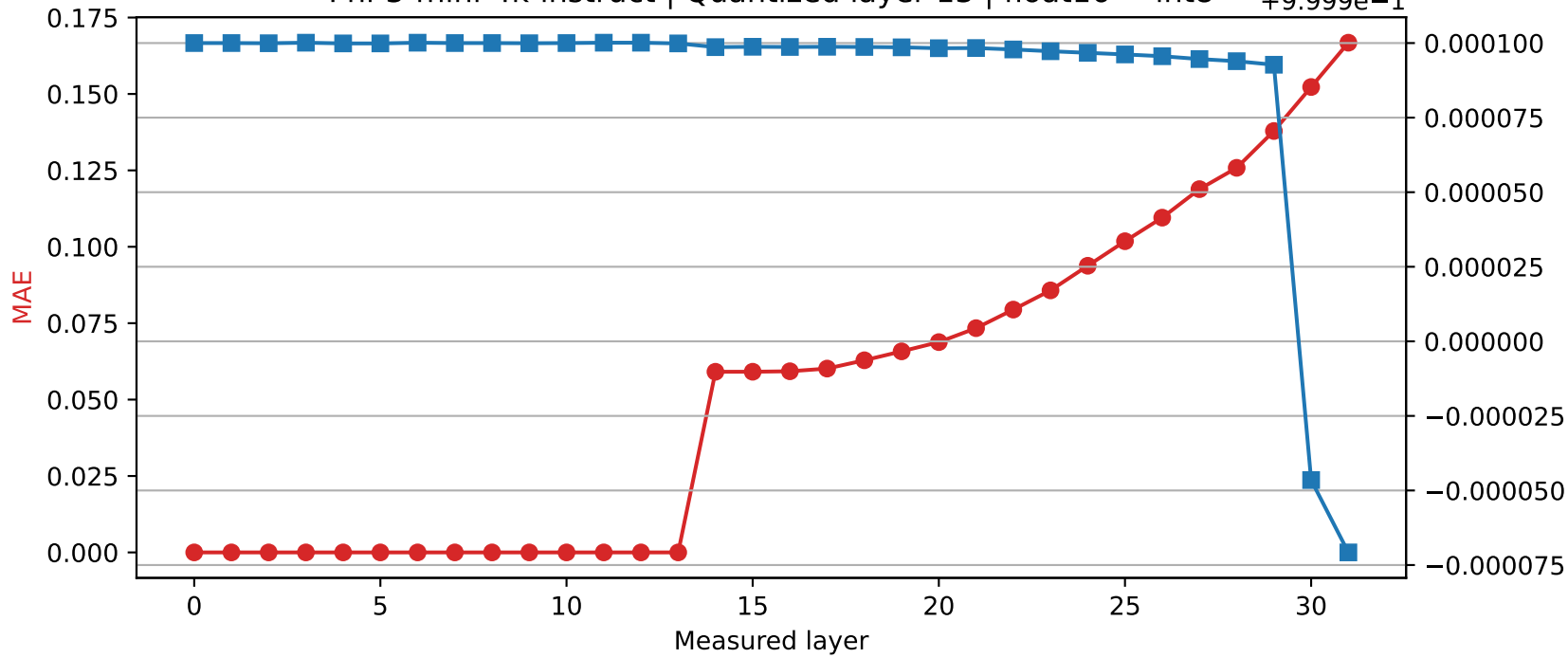
Phi-3-mini-4k-instruct | Quantized layer 13 | float16 → int8
