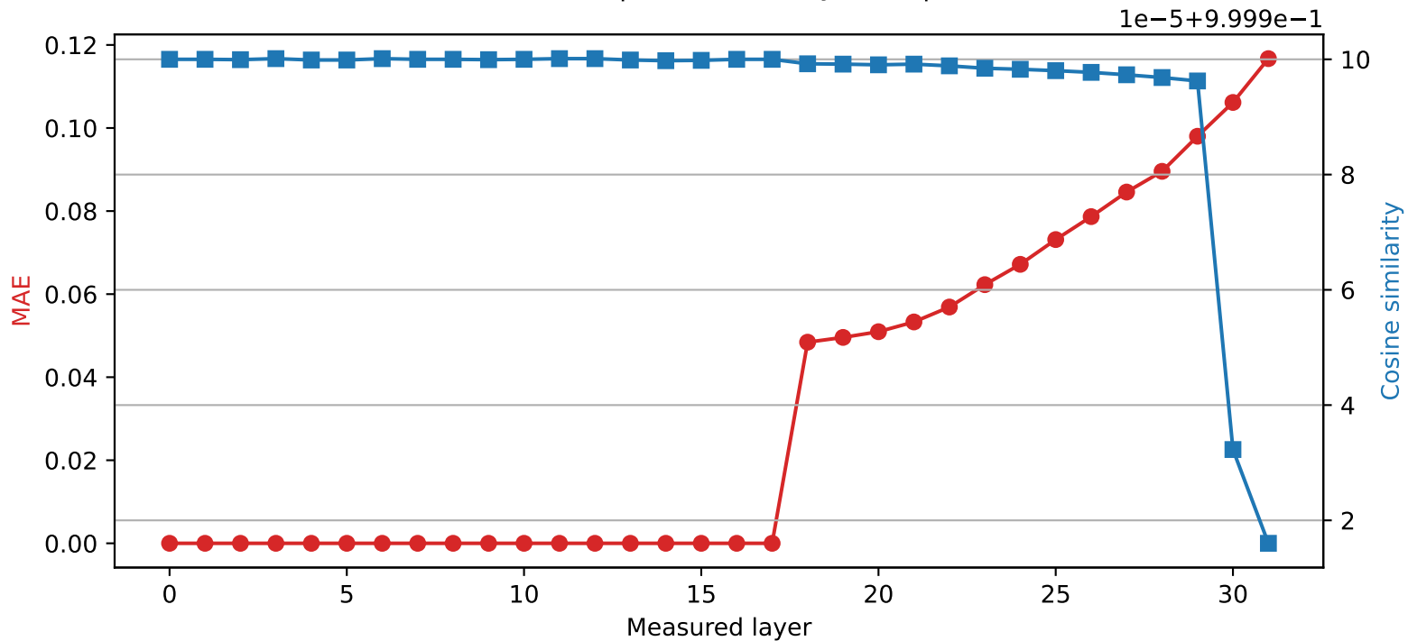
Phi-3-mini-4k-instruct | Quantized layer 17 | float16 → int8
