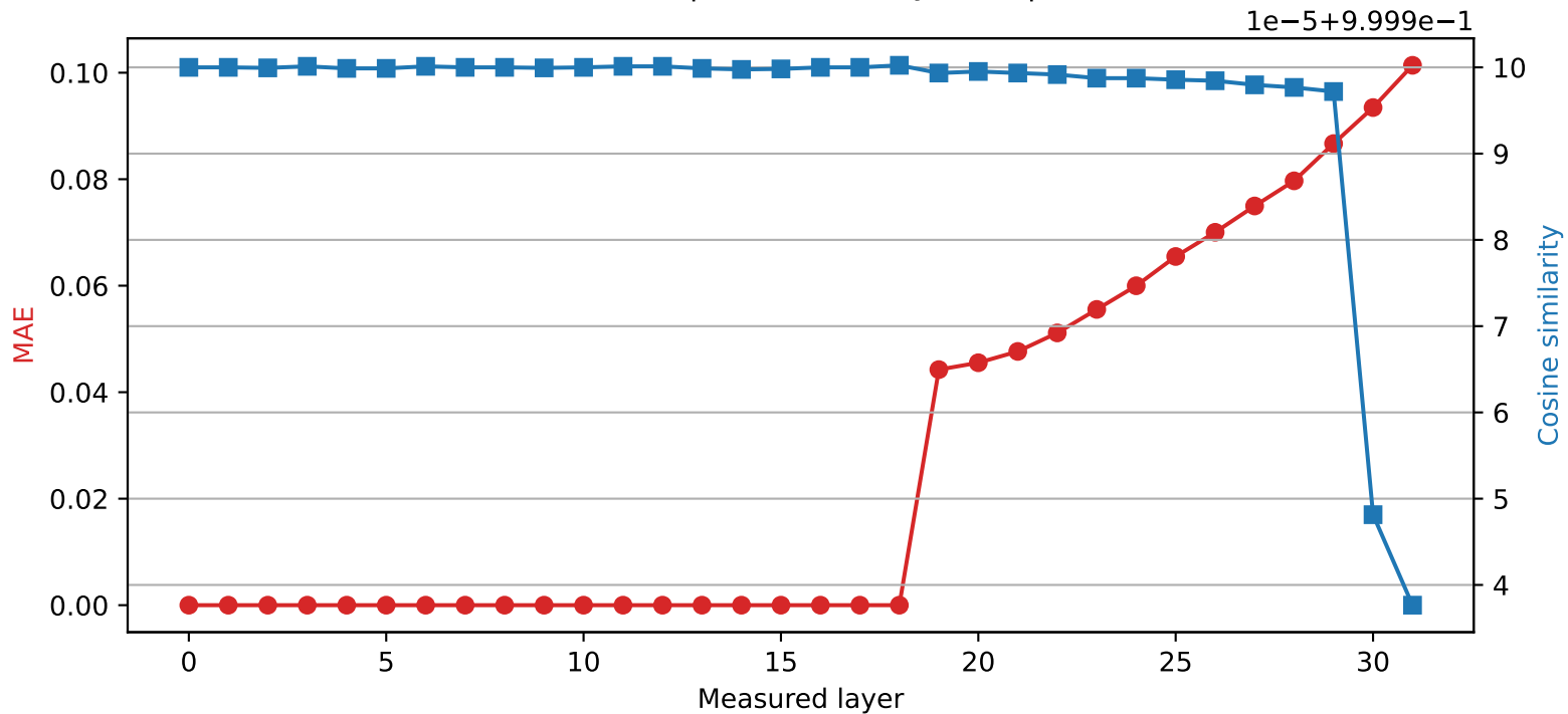
Phi-3-mini-4k-instruct | Quantized layer 18 | float16 → int8
