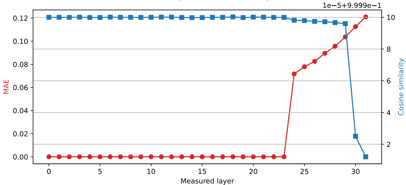
Phi-3-mini-4k-instruct | Quantized layer 23 | float16 \rightarrow int8
