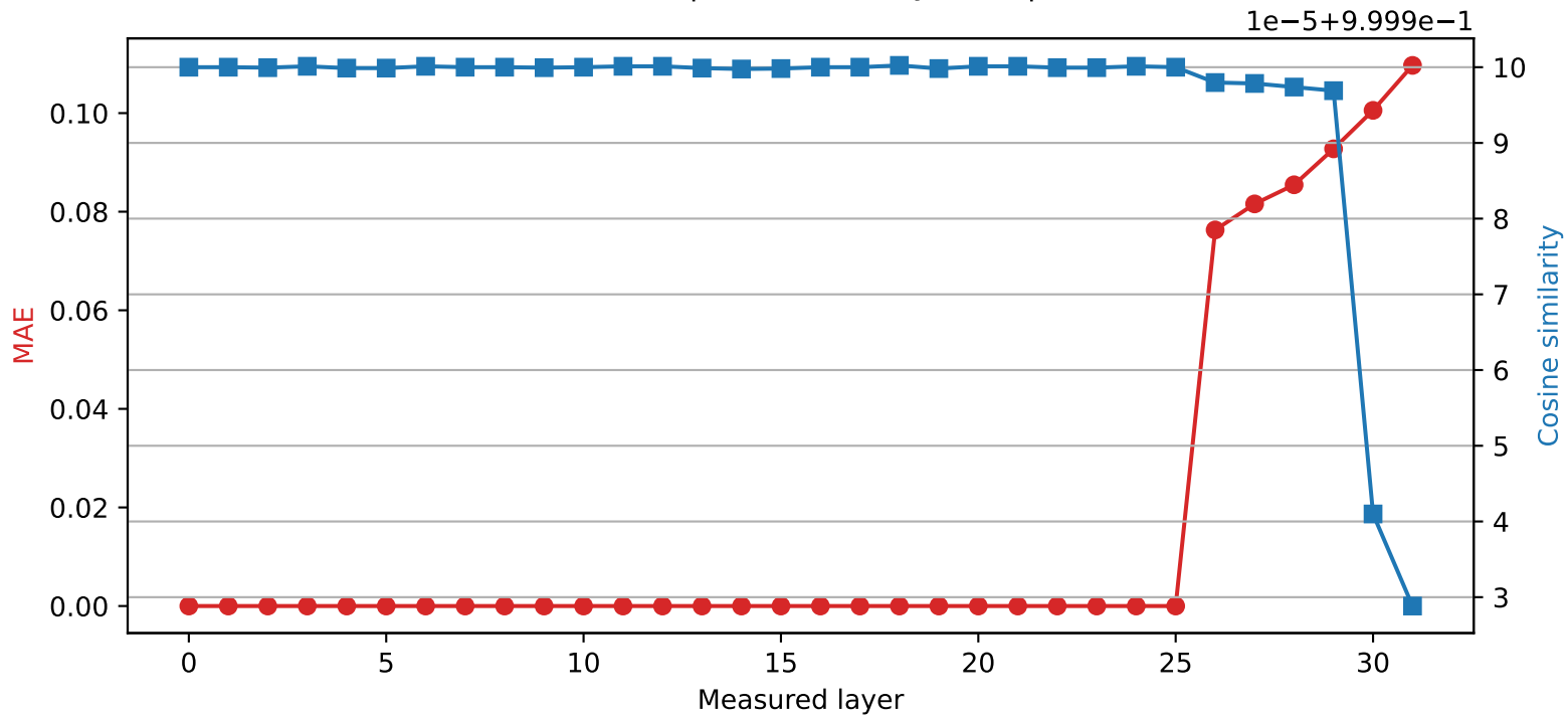
Phi-3-mini-4k-instruct | Quantized layer 25 | float16 → int8
