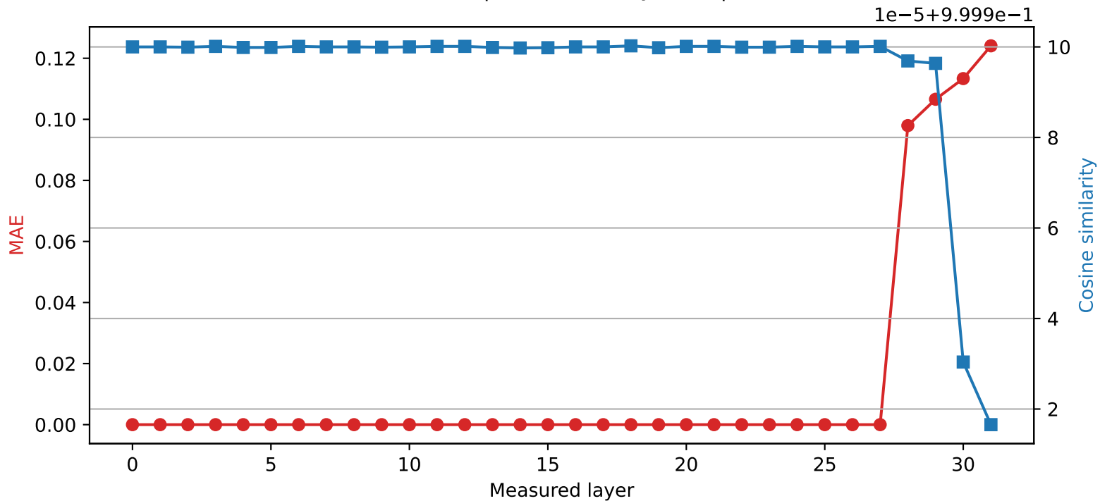
Phi-3-mini-4k-instruct | Quantized layer 27 | float16 \rightarrow int8
