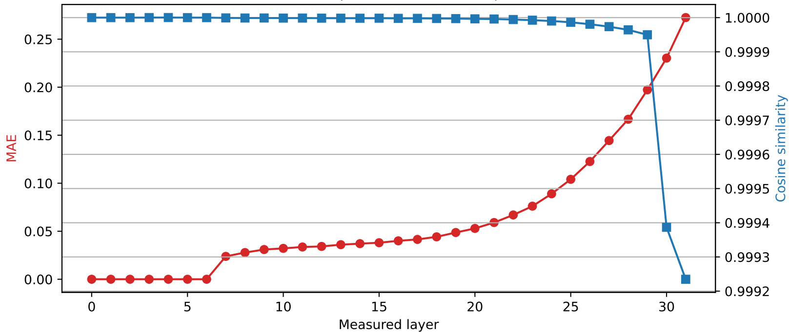
Phi-3-mini-4k-instruct | Quantized layer 6 | float16 \rightarrow int8
