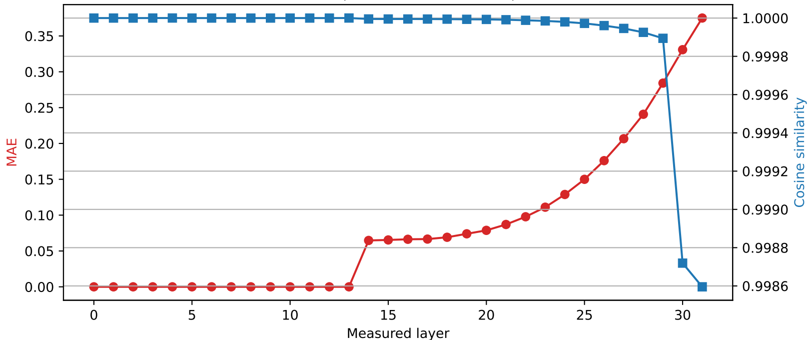
Phi-3-mini-4k-instruct | Quantized layer 13 | float16 \rightarrow int8
