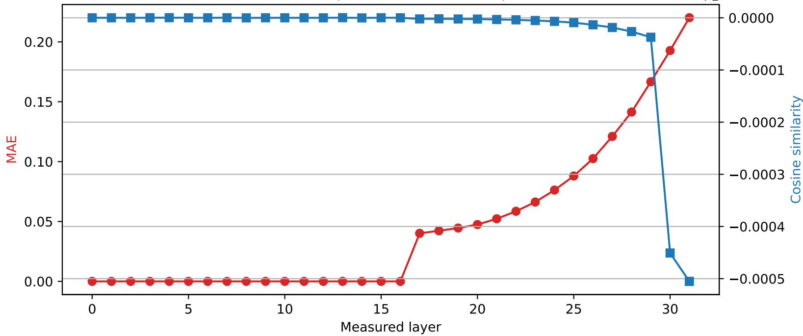
Phi-3-mini-4k-instruct | Quantized layer 16 | float16 \rightarrow int8
