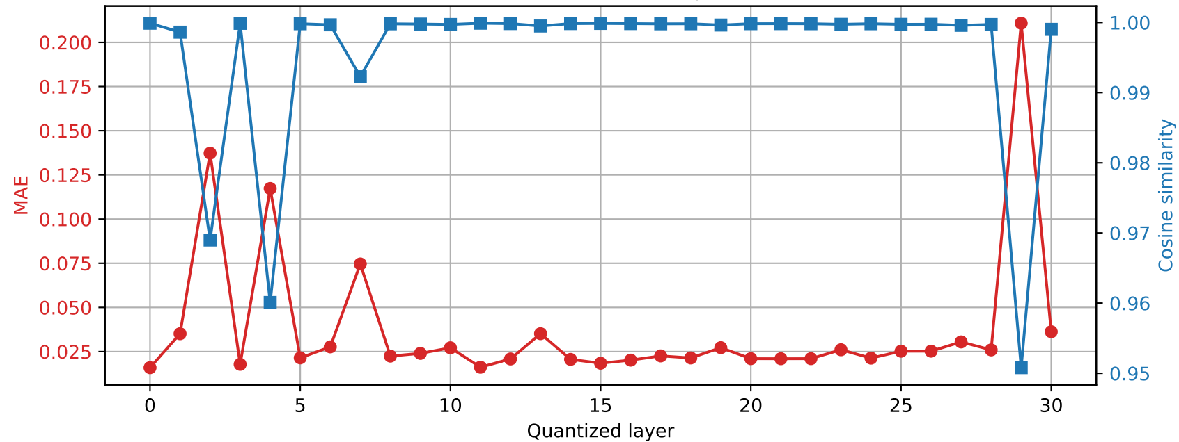
Phi-3-mini-4k-instruct | Prompt 2 Final RMSNorm output damage | float16 \rightarrow int8
