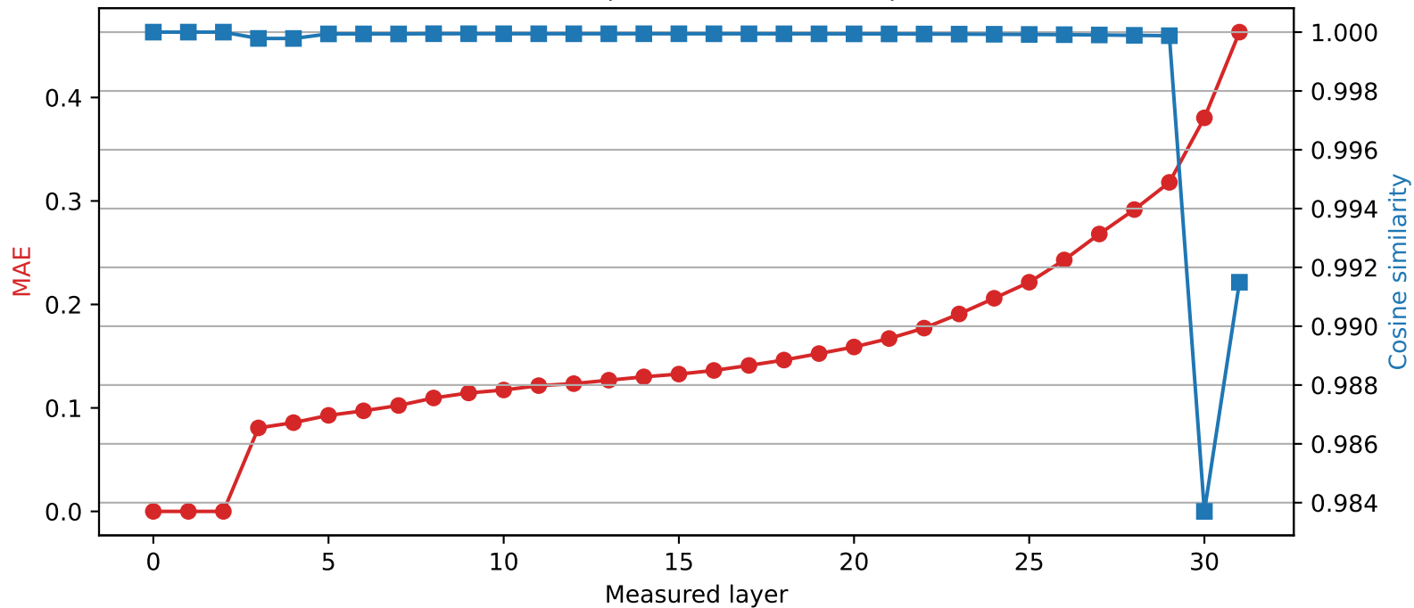
Phi-3-mini-4k-instruct | Quantized layer 2 | float16 \rightarrow int8
