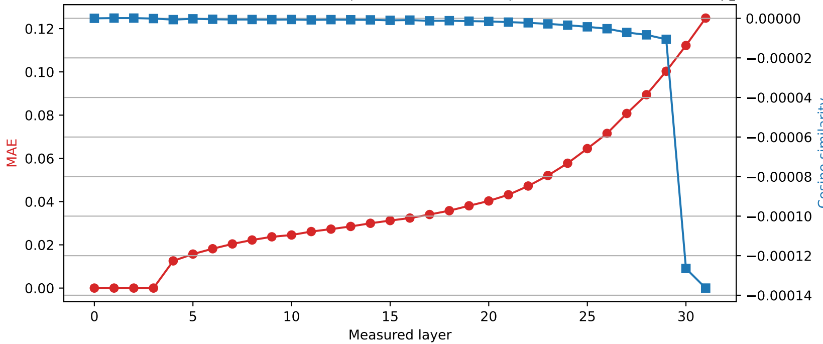
Phi-3-mini-4k-instruct | Quantized layer 3 | float16 \rightarrow int8
