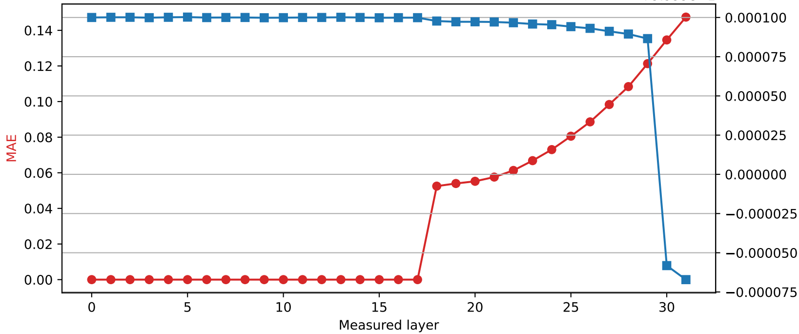
Phi-3-mini-4k-instruct | Quantized layer 17 | float16 → int8
