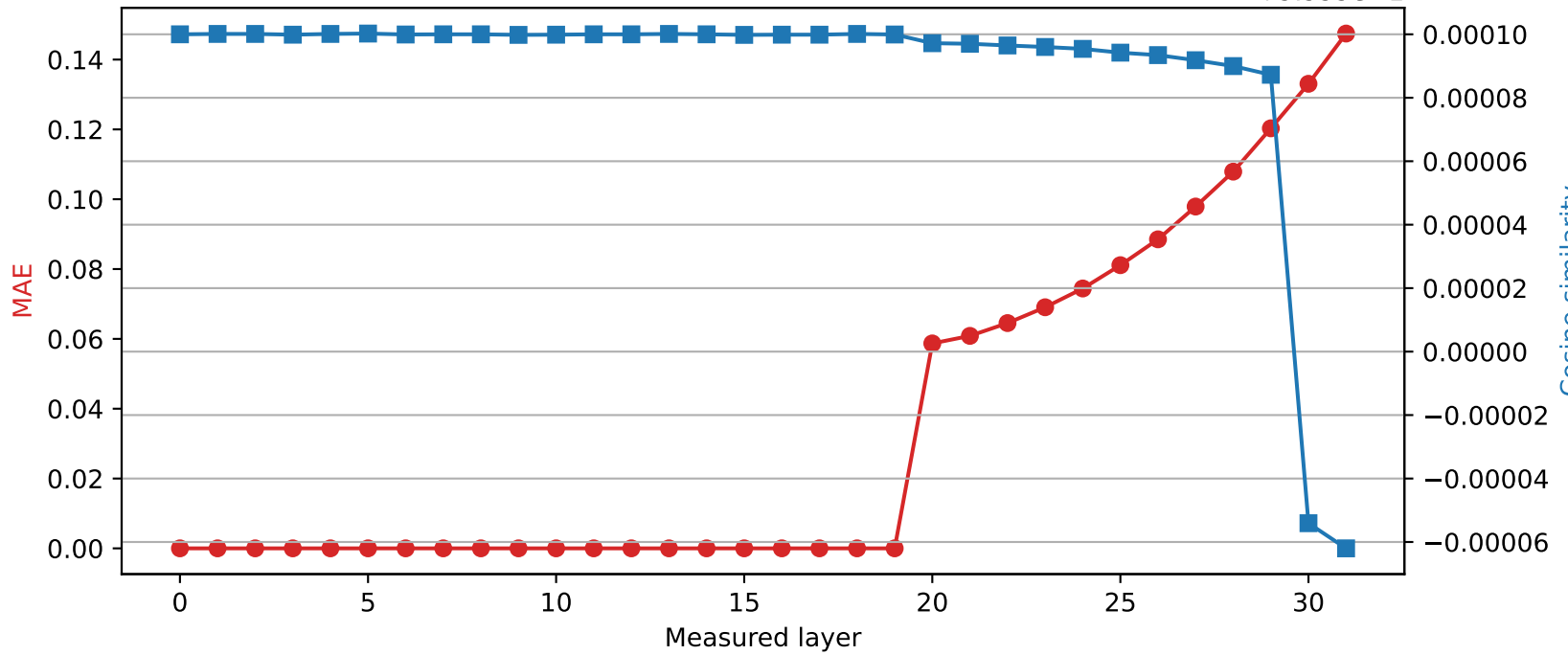
Phi-3-mini-4k-instruct | Quantized layer 19 | float16 → int8
