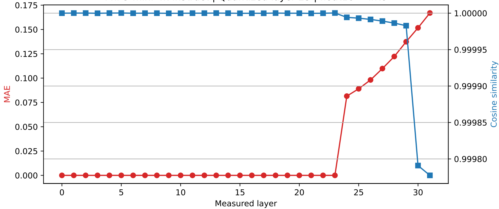
Phi-3-mini-4k-instruct | Quantized layer 23 | float16 \rightarrow int8
