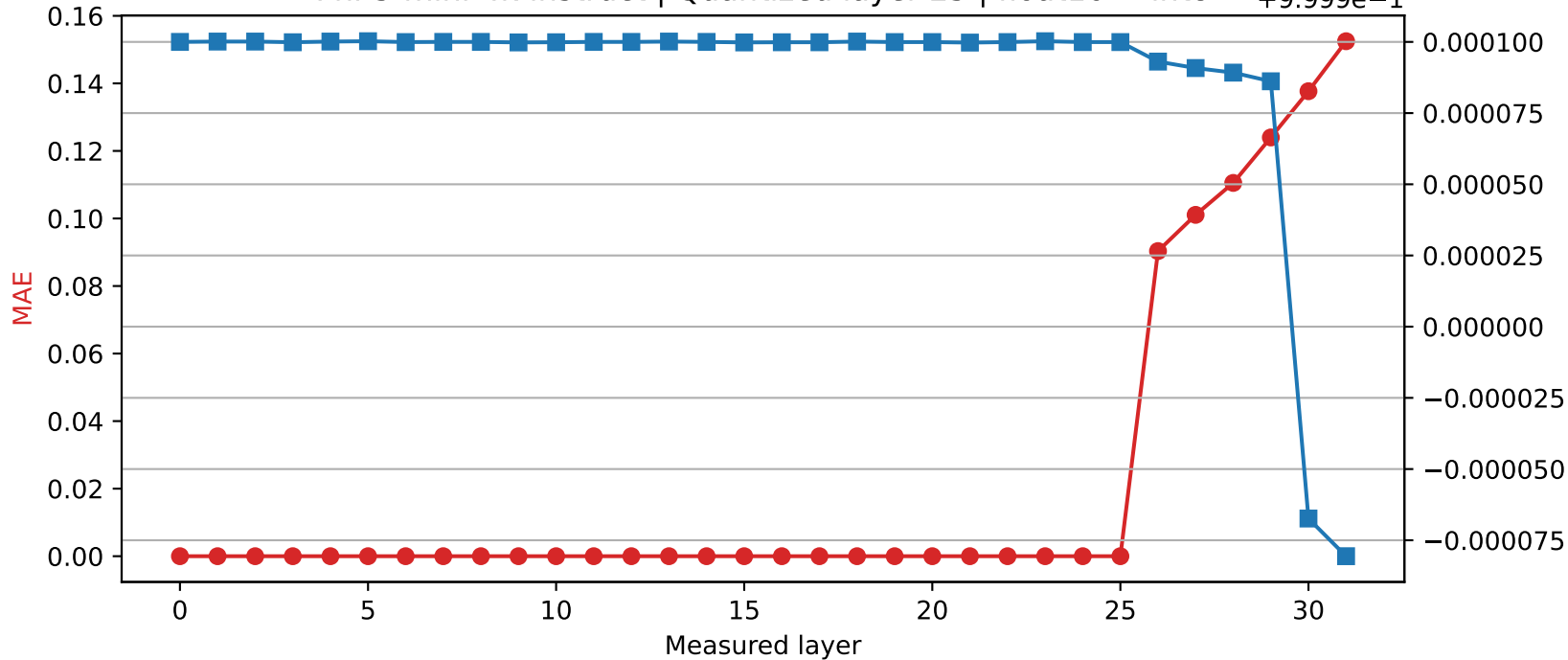
Phi-3-mini-4k-instruct | Quantized layer 25 | float16 → int8
