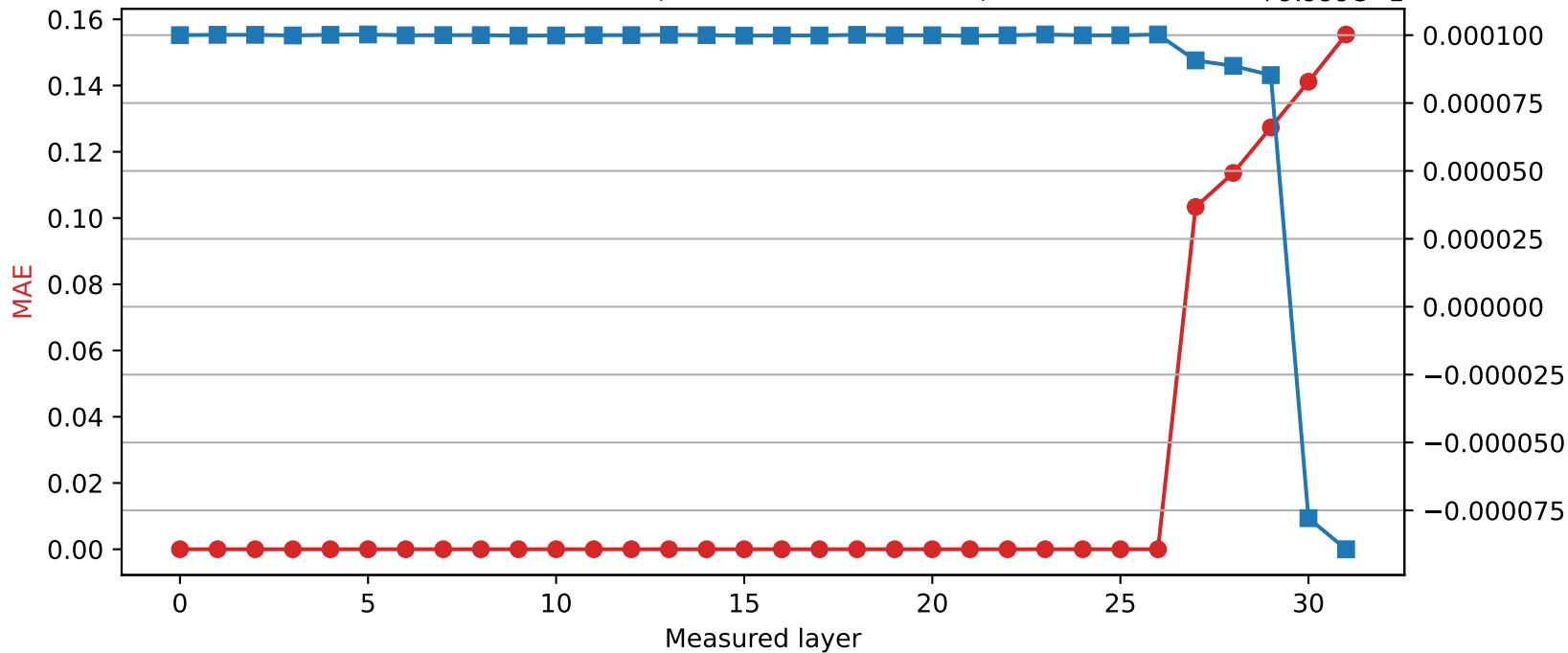
Phi-3-mini-4k-instruct | Quantized layer 26 | float16 → int8
