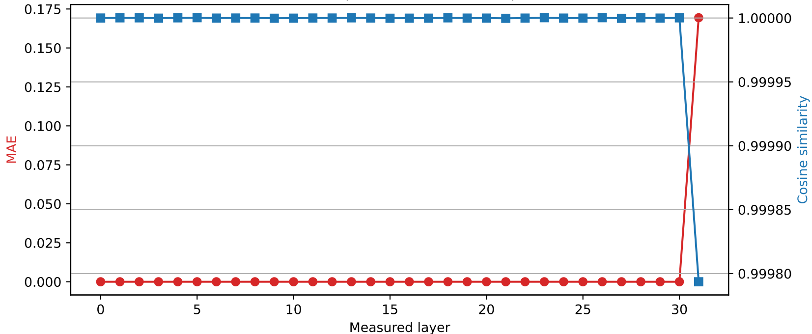
Phi-3-mini-4k-instruct | Quantized layer 30 | float16 \rightarrow int8
