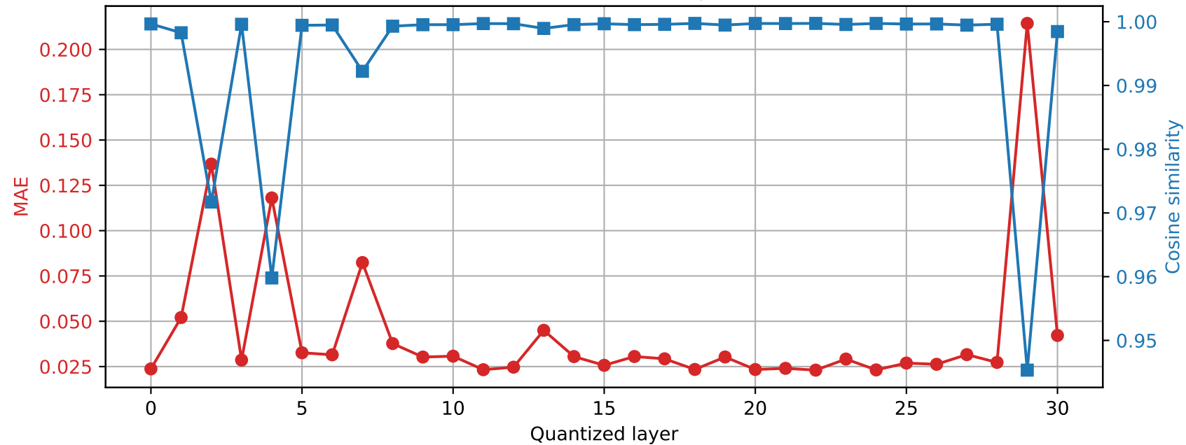
Phi-3-mini-4k-instruct | Prompt 3 Final RMSNorm output damage | float16 \rightarrow int8
