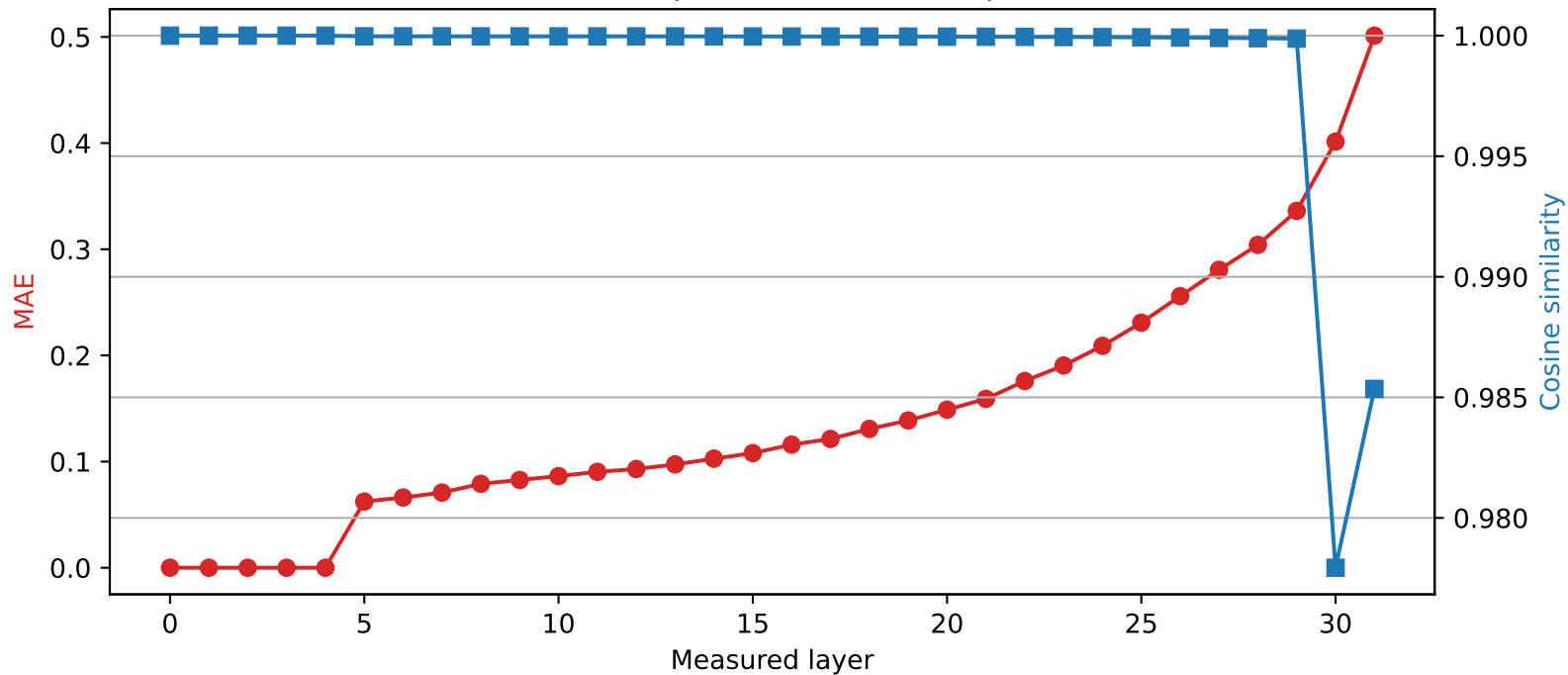
Phi-3-mini-4k-instruct | Quantized layer 4 | float16 \rightarrow int8
