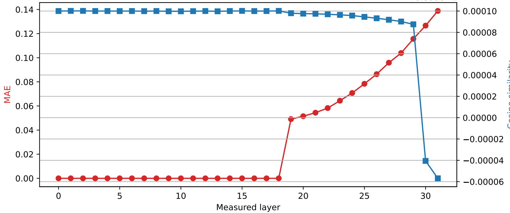
Phi-3-mini-4k-instruct | Quantized layer 18 | float16 → int8
