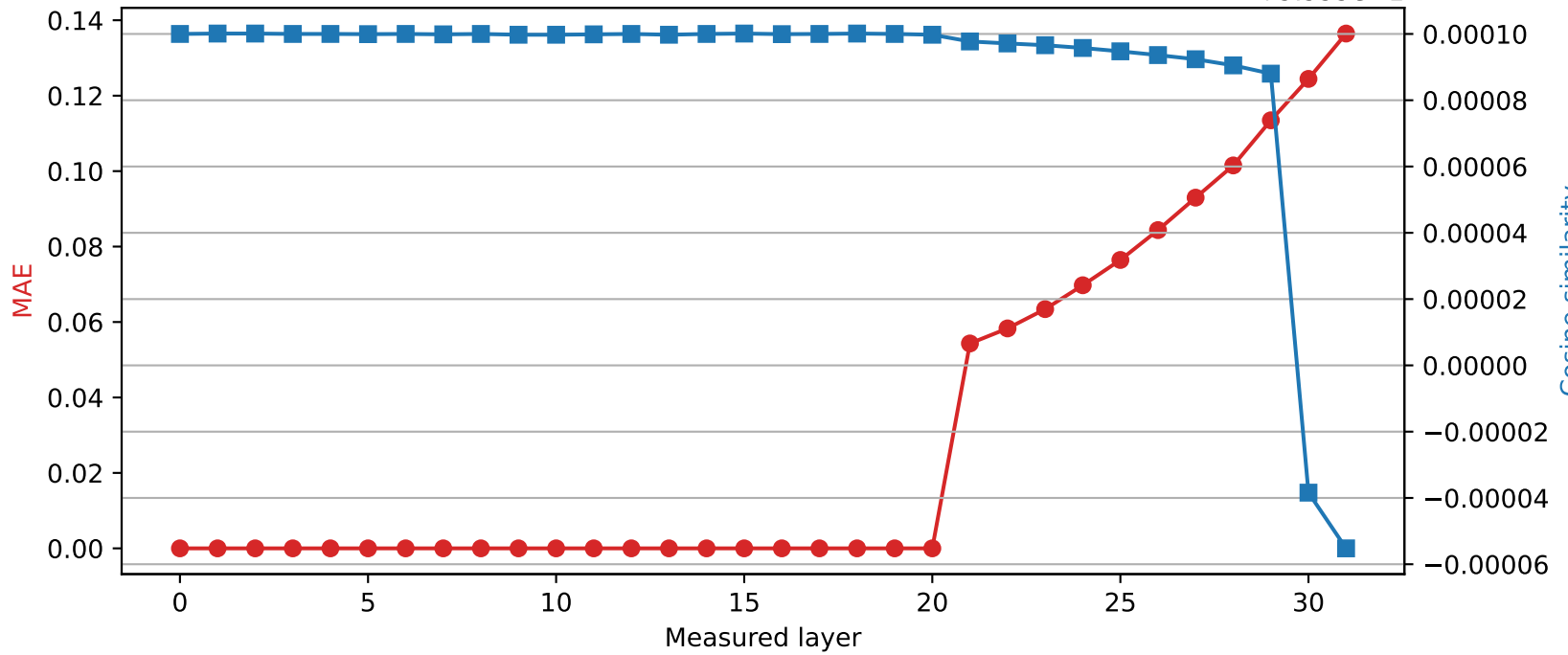
Phi-3-mini-4k-instruct | Quantized layer 20 | float16 → int8
