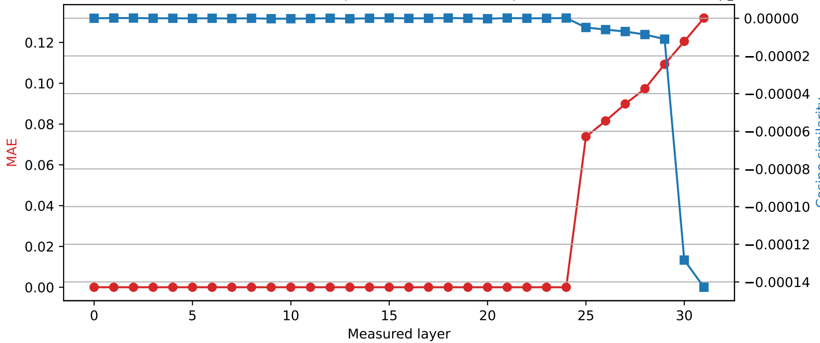
Phi-3-mini-4k-instruct | Quantized layer 24 | float16 \rightarrow int8
