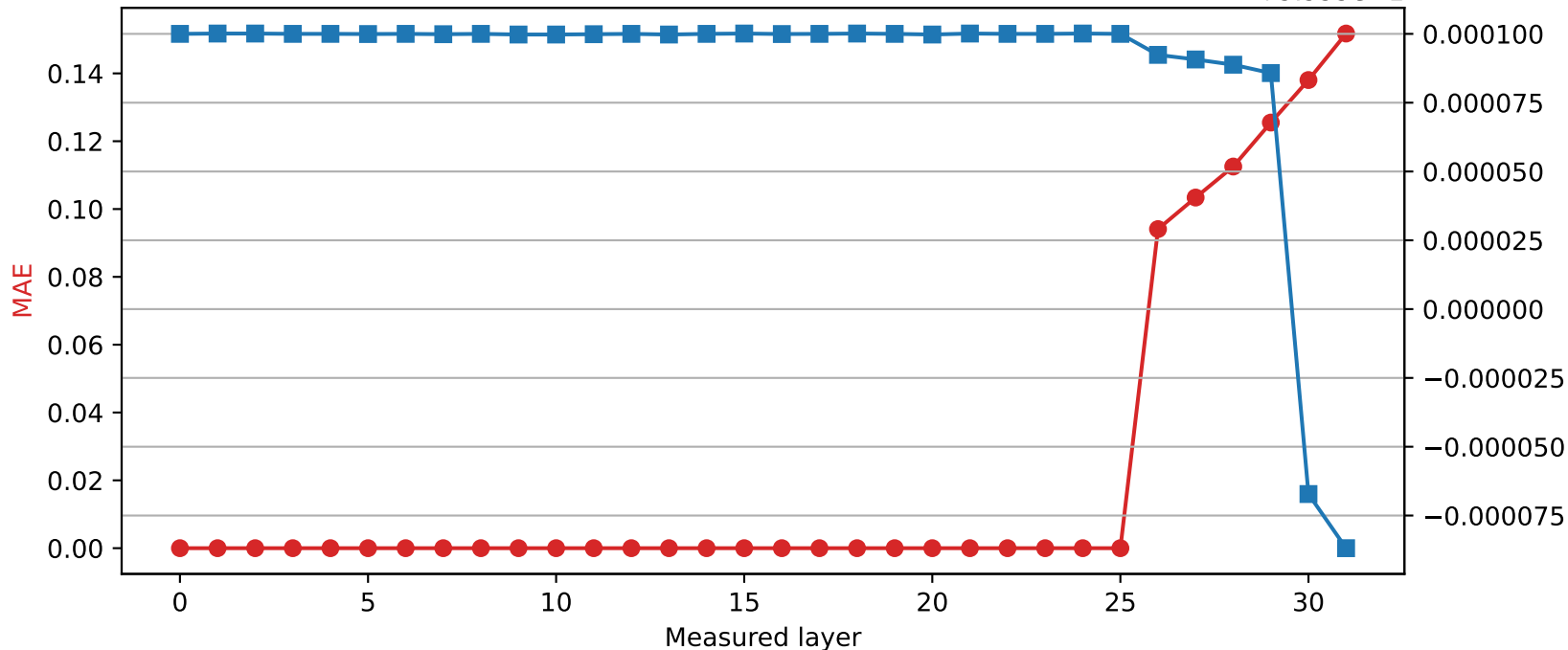
Phi-3-mini-4k-instruct | Quantized layer 25 | float16 \rightarrow int8
