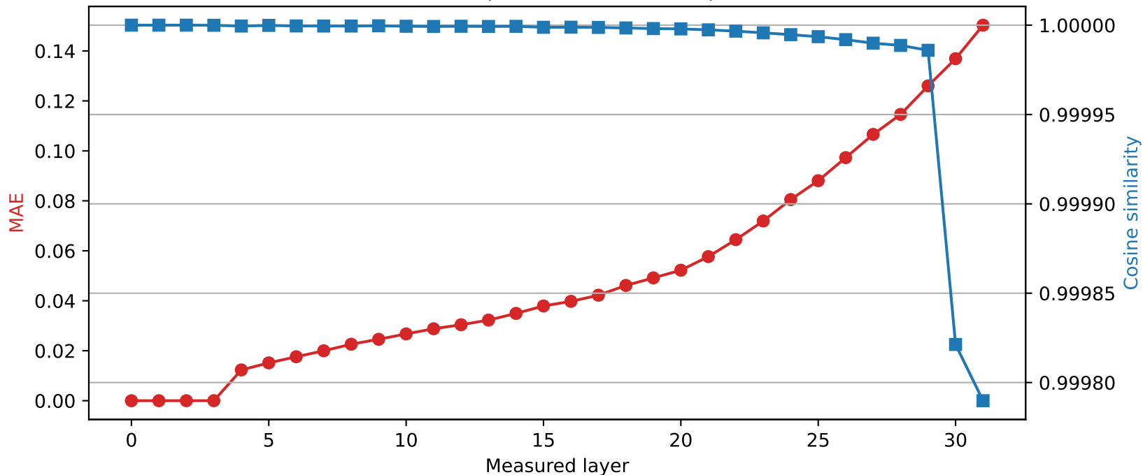
Phi-3-mini-4k-instruct | Quantized layer 3 | float16 \rightarrow int8
