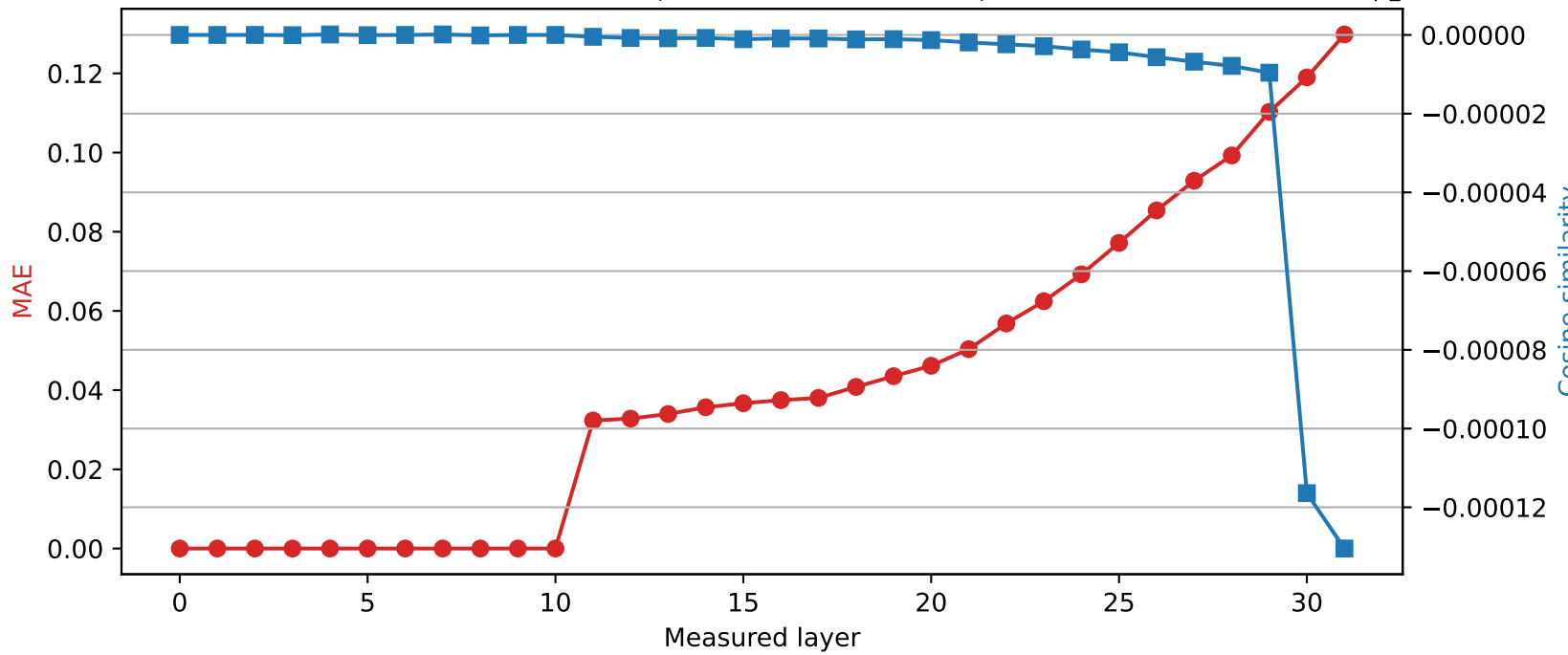
Phi-3-mini-4k-instruct | Quantized layer 10 | float16 \rightarrow int8
