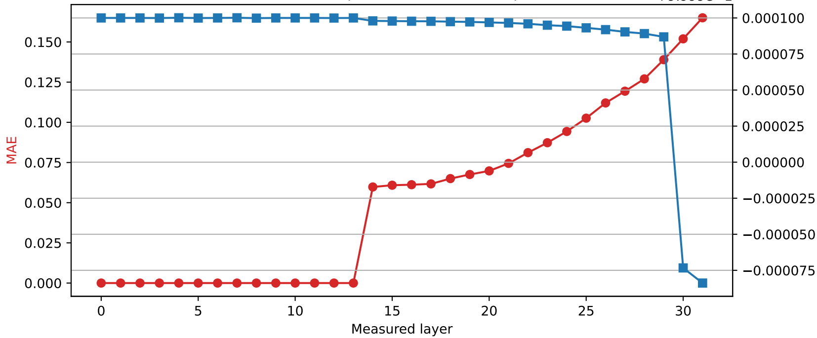
Phi-3-mini-4k-instruct | Quantized layer 13 | float16 \rightarrow int8
