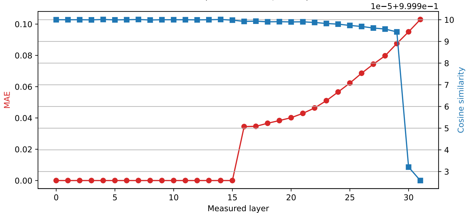
Phi-3-mini-4k-instruct | Quantized layer 15 | float16 → int8
