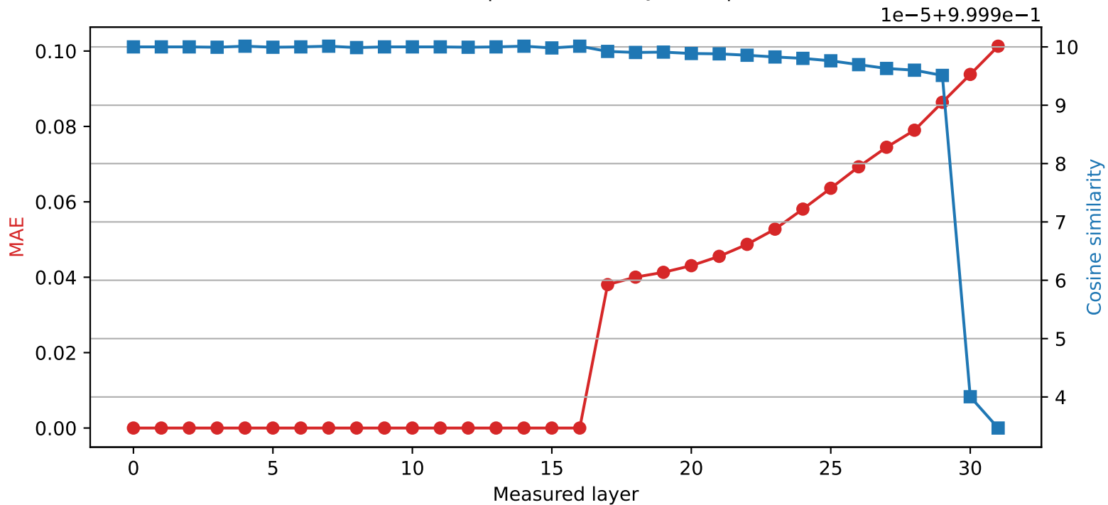
Phi-3-mini-4k-instruct | Quantized layer 16 | float16 → int8
