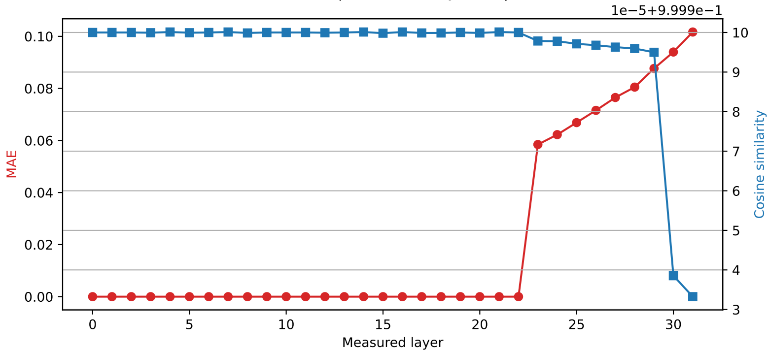
Phi-3-mini-4k-instruct | Quantized layer 22 | float16 \rightarrow int8
