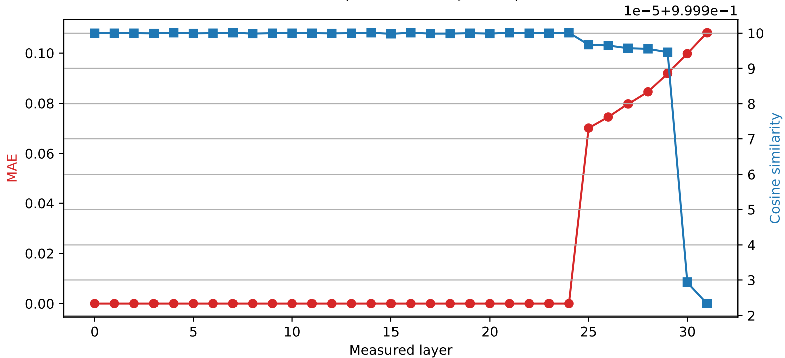
Phi-3-mini-4k-instruct | Quantized layer 24 | float16 → int8
