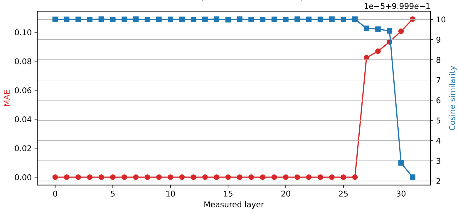
Phi-3-mini-4k-instruct | Quantized layer 26 | float16 \rightarrow int8
