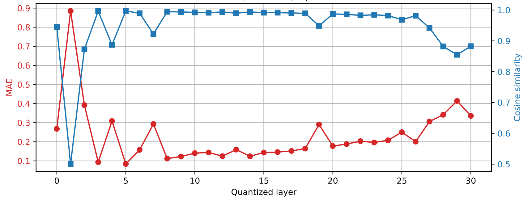
Phi-3-mini-4k-instruct | Prompt 0 Final RMSNorm output damage | float16 \rightarrow int4
