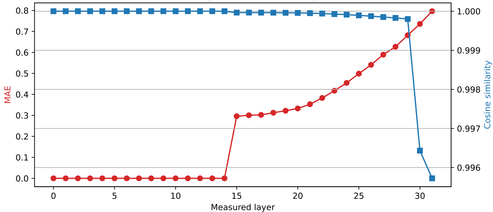
Phi-3-mini-4k-instruct | Quantized layer 14 | float16 \rightarrow int4
